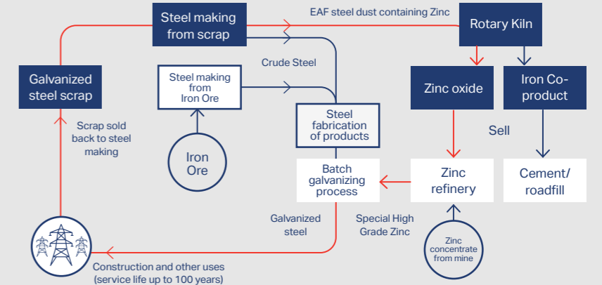
Recovery of zinc from galvanized steel, without loss of properties, after many decades of service
